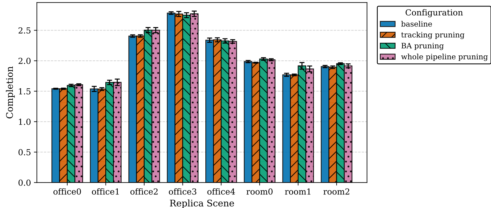
Completion ( \downarrow ) across Replica Scenes (Mean & Std Dev)
